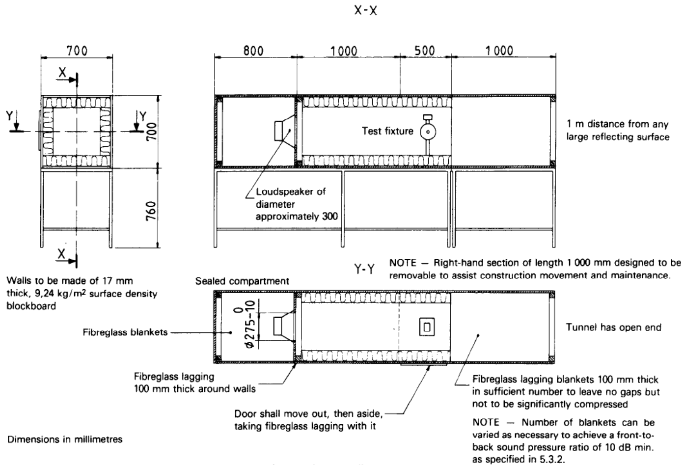
Figure 2 — Example of a test site arrangement (acoustic tunnel)
